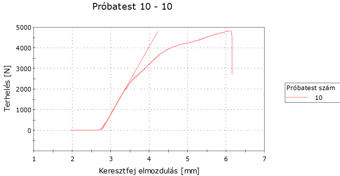
Figures A-39 to -48 Load-displacement curves. TBWD-type specimens, withdrawal test
