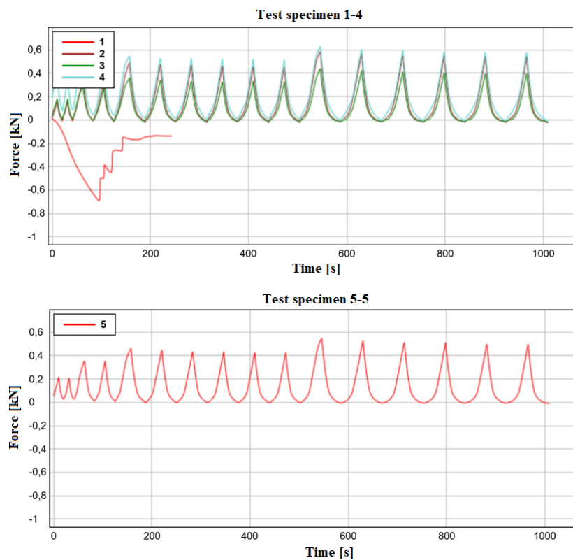
Figure 3.17 Force vs. load cycle diagram of the specimens tested
