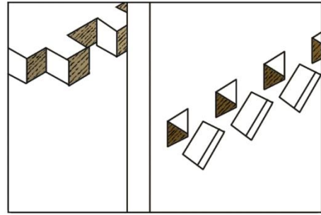
Figure 1.12. Pinned Mortise& Tennon Joint (drawing by S.Baş)
