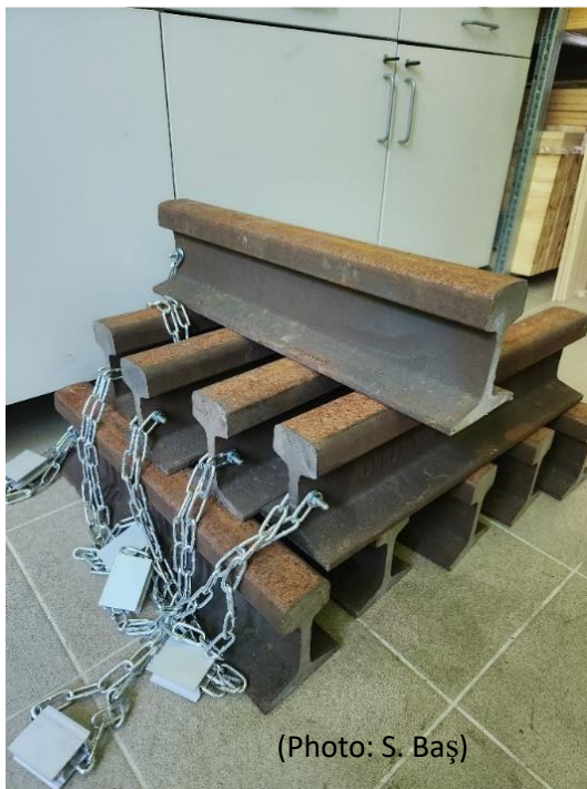
Figure 2.9 Weights used in the creep test for the big test pieces
