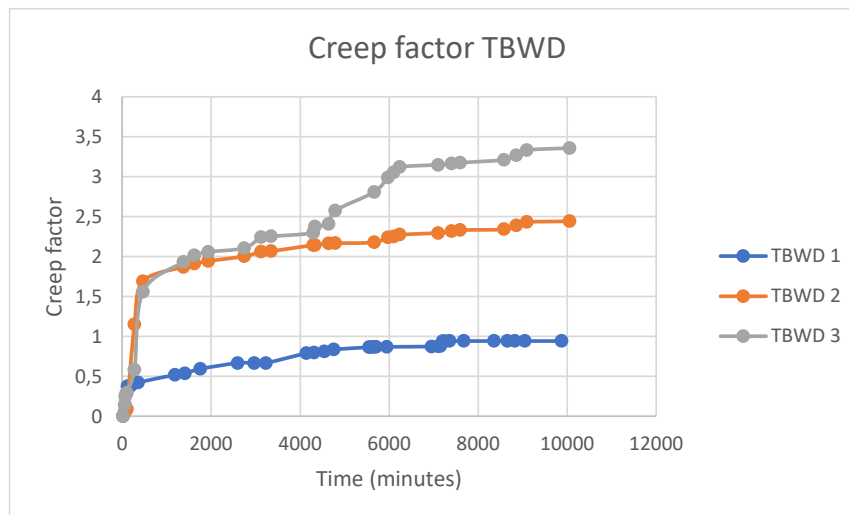
Figure 3.23 Creep curves of TBWD – type specimens
