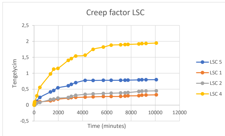
Figure 3.26 Creep curves of LSC – type specimens
