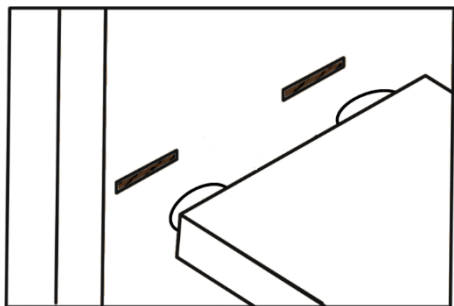
Figure 1.14 Biscuit Joint (drawing by S.Baş)
