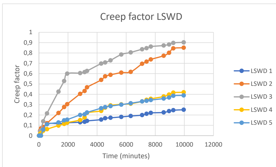
Figure 3.22 Creep curves of LSWD – type specimens
