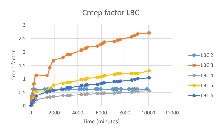
Figure 3.25 Creep curves of LBC – type specimens
