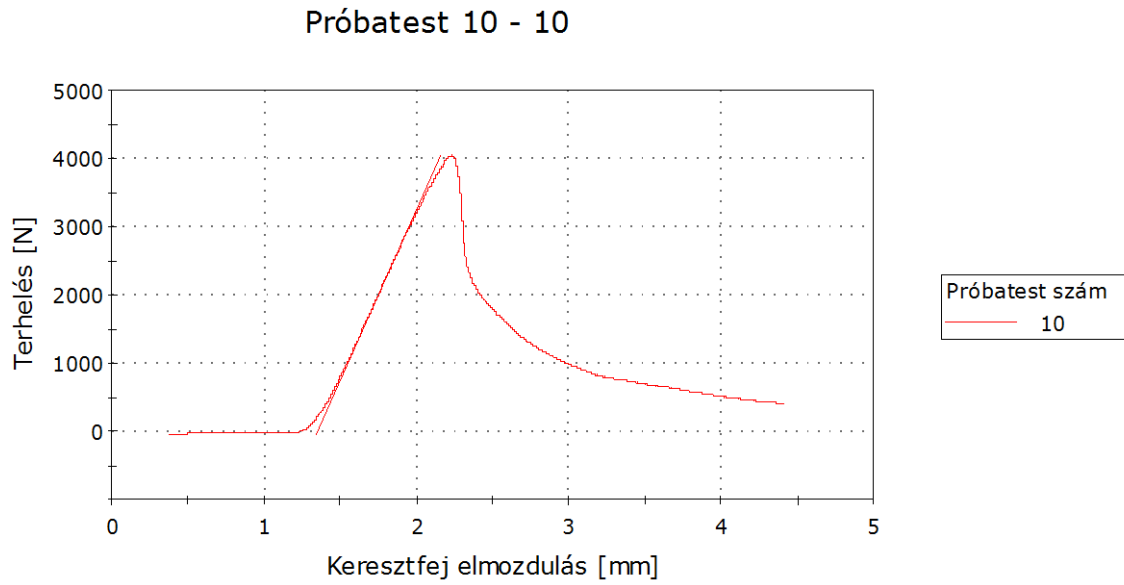
Figures A-29 to -38 Load-displacement curves. TBWD-type specimens, withdrawal test
