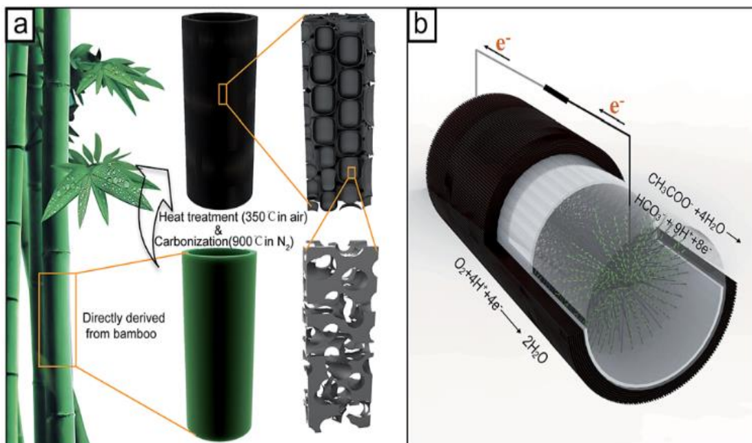
Figure 1.12 (a) Fabrication process of the cathode from a bamboo tube; (b) MFC with a cathode made from the bamboo tube. (Published from Ref. Yang et al., (2017) under CC BY 3.0 license).
