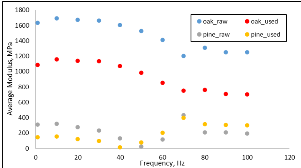
Figure 3.20 Average elastic modulus versus frequency for 4 mm wall thickness oak and Scots pine at constant temperature (25 °C) and humidity (14% RH). Blue dots are raw-oak before use in the samples. The red dots are oak after three months of continuous use. Grey dots are raw-Scots pine before use in the samples. Yellow dots are Scots pine after 3 months of continuous use.
