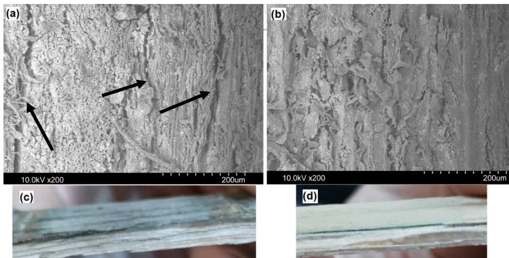
Figure 3.21 SEM micrographs of the inner surface of 4 mm wall thickness WML-MFC after three months of use from (a) oak (b) Scots pine. Digital photographs from the container wall show the inner surface cross-section and the side view of (c) oak (d) Scots pine.
