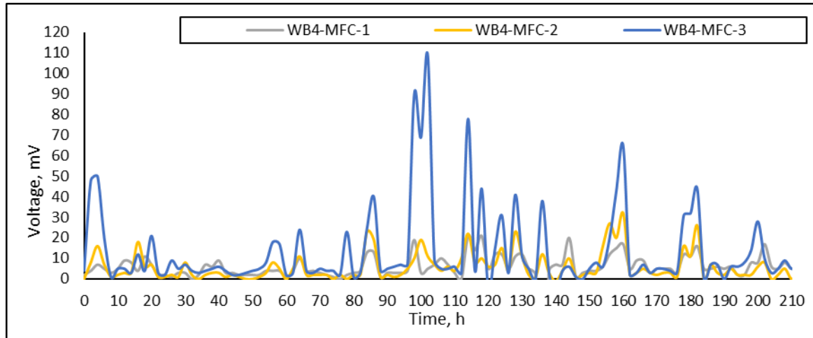
Figure 3.1 Voltage of black locust containers during the last 210 h after 90 days of operating with open circuit condition.
