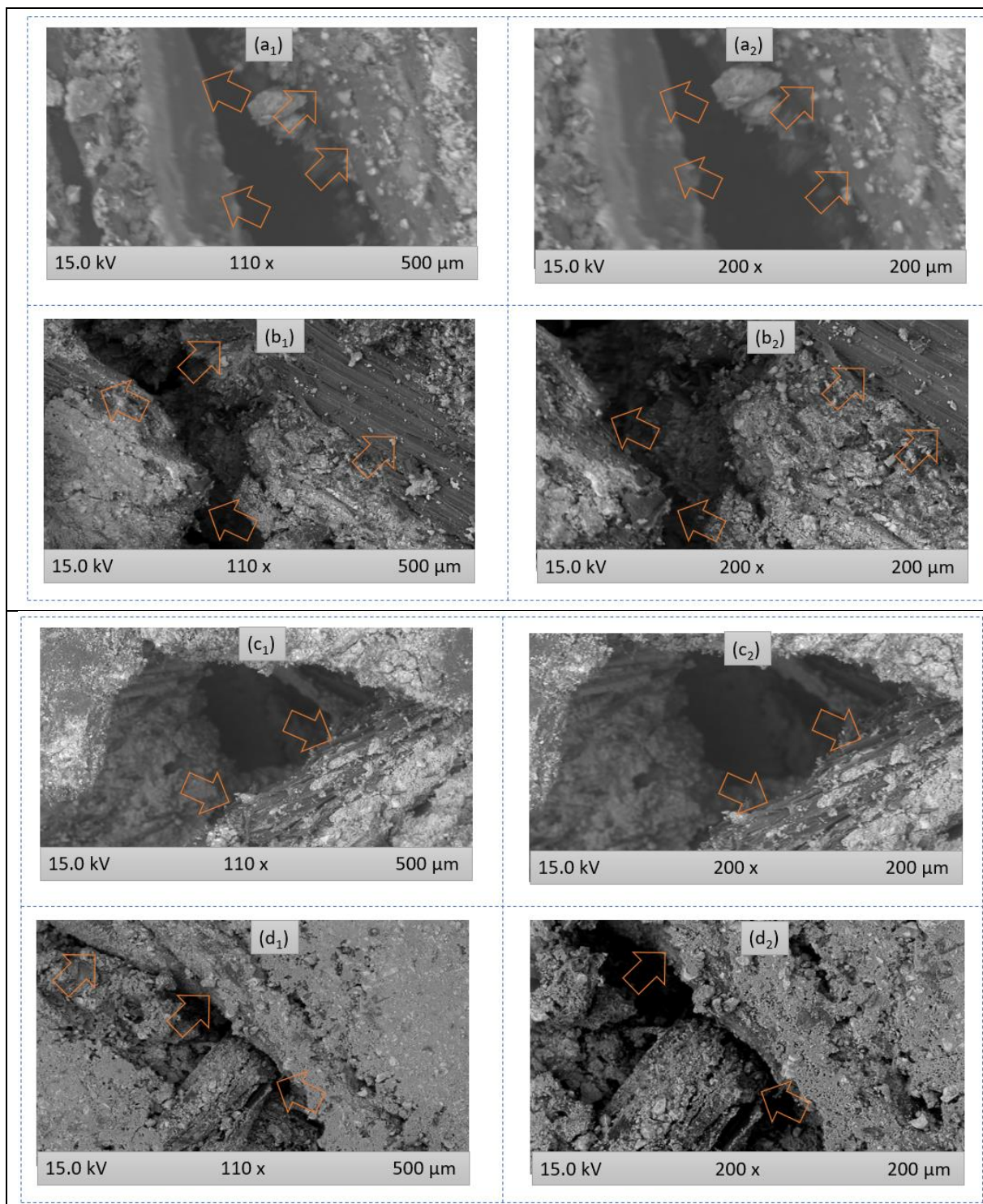
Figure 5.9: SEM micrographs of specimens (before fracture) of produced composite panels from coir fiber and scots pines reinforced with OPC: P@C1 (a 1 and a 2 ), PC@C2 (b 1 and b 2 ), PC@C3 (c 1 and c 2 ), PC@C4 (d 1 and d 2 ), and C@C5 (e 1 and e 2 ).
