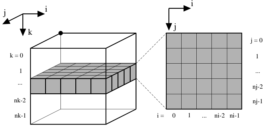
Figure 2-10. The 3D voxel space is composed of a set of 2D rasters. The cells are identified by the indices of columns ( i ), rows ( j ) and planes ( k ).
