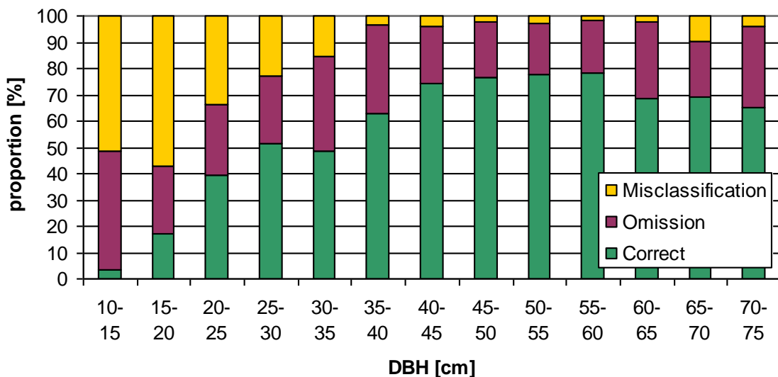
Figure 5-7. Performance of tree detection based on 2D image objects in different DBH classes.
