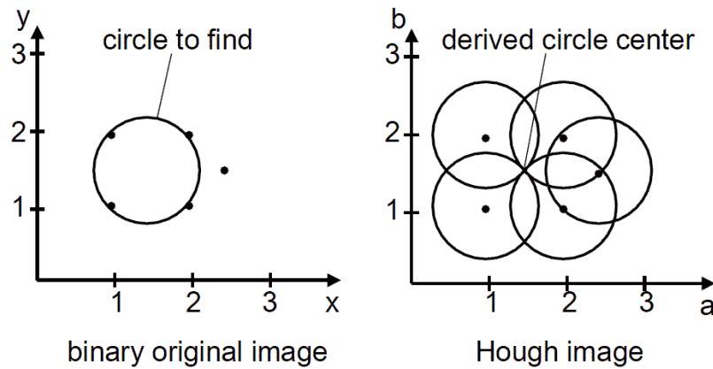
Figure 2-21. Concept of Hough-transformation for circle detection (Simonse et al., 2003).
