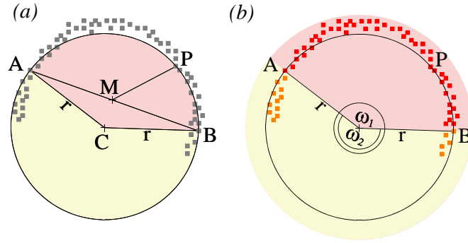
Figure 4-17. Calculation of the filter value for the selection of circular objects.
