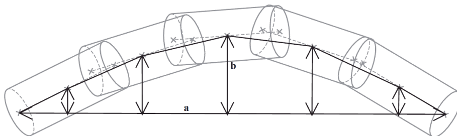
Figure 2-23. Fitted cylinders in telescopic arrangement, the approximated tree axis as the connections of cylinder axis centres, a chord (a) and the corresponding pitch (b). (Thies et al., 2004)
