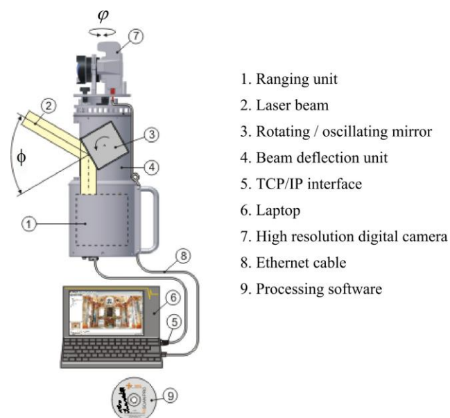
Figure 2-4. The main components of laser scanner system on the example of Riegl LMS Z420i (www.riegl.com).
