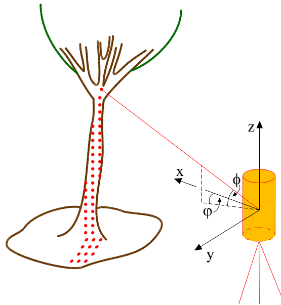
Figure 2-6. Raw observables in the sensor's own coordinate system.
