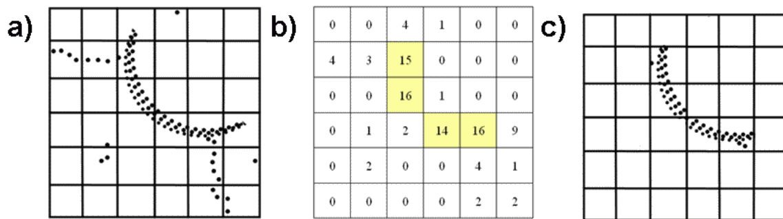
Figure 2-18. Filtering for single scans by elimination of cells with few measurements (Bienert et al, 2007). The threshold of minimum point counts is 13 per cells in this example, which was computed upon the scanning resolution and the target distance.
