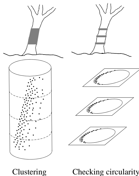
Figure 4-14. Point slice used for the clustering and its sub-sections for checking the circularity of the clusters.
