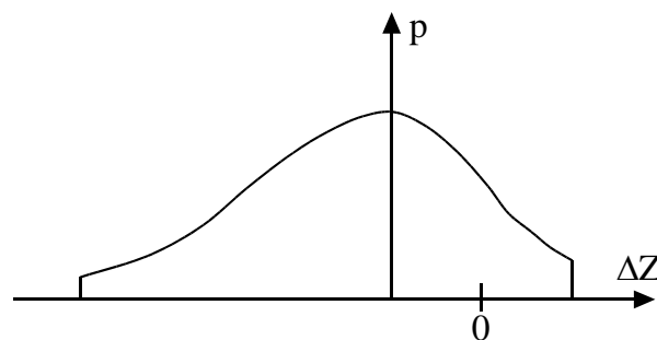
Figure 2-15. Weight function for filtering terrain points. (Kraus and Pfeifer, 1998)
