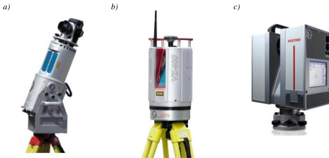
Figure 2-5. Examples on recent terrestrial laser scanners a) Riegl LMS-Z 420i (pulse ranging) b) Riegl VZ400 (pulse ranging with full waveform digitization) c) Leica HDS7000 (phase shift) ( www.riegl.com , www.leica-geosystems.com ).
