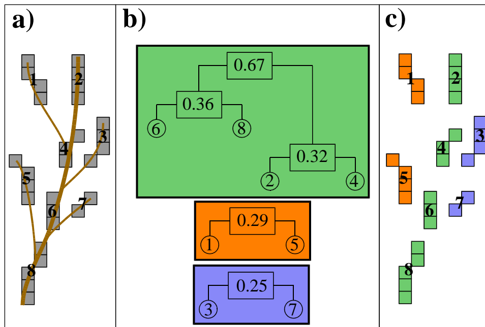
Figure 4-25. Aggregation of generalized objects representing a juvenile tree stem and branches (a). The procedure is accomplished in five steps where the objects of those are aggregated that resulted in the maximum value of A (b). The largest disconnected voxel object represents the stem being reconstructed from four fragments (c).
