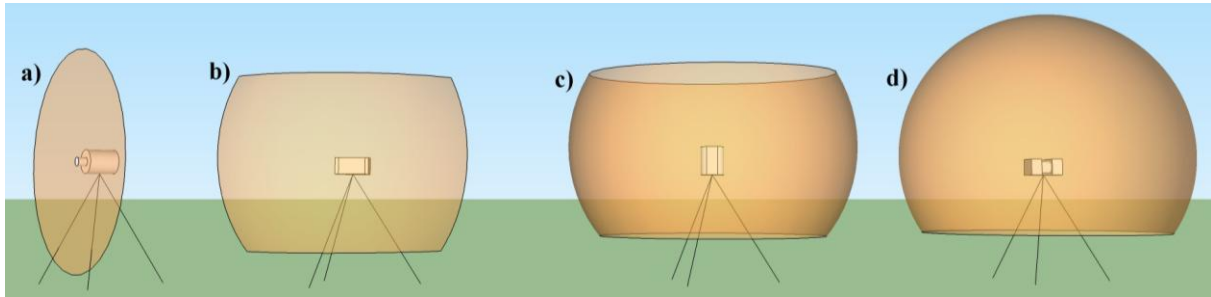
Figure 2-3. Scanners' field of view: (a) line scanner (b) frame scanner (c) panoramic scanner with limited upper zenith angle (d) panoramic scanner with full view over the upper hemisphere. (Illustrated by the author)
