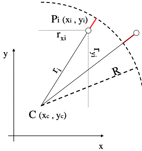
Figure 4-15. Notations for the geometric circle fit.
