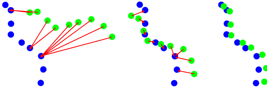
Figure 2-8. Concept of the ICP algorithm illustrated in three iterative steps. (Adapted from Pfeifer, 2007)
