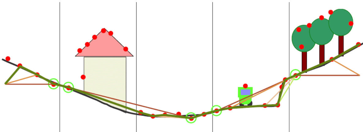
Figure 2-14. Progressive TIN densification (Mandelburger, 2005).
