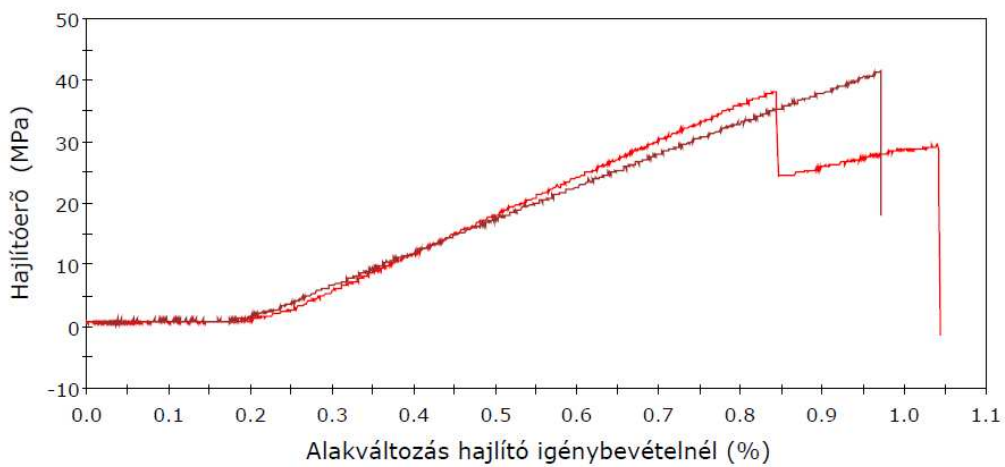
Flex Test
