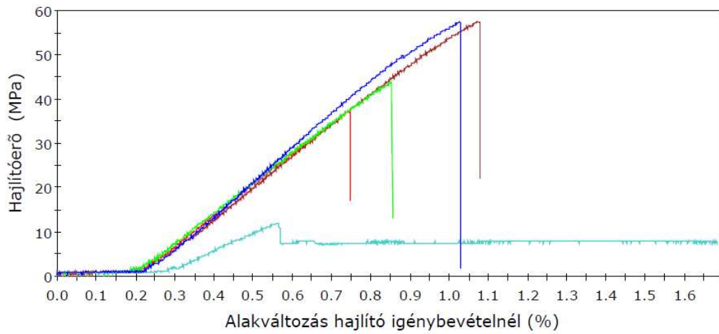
Flex Test
