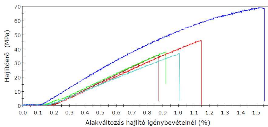
Flex Test
