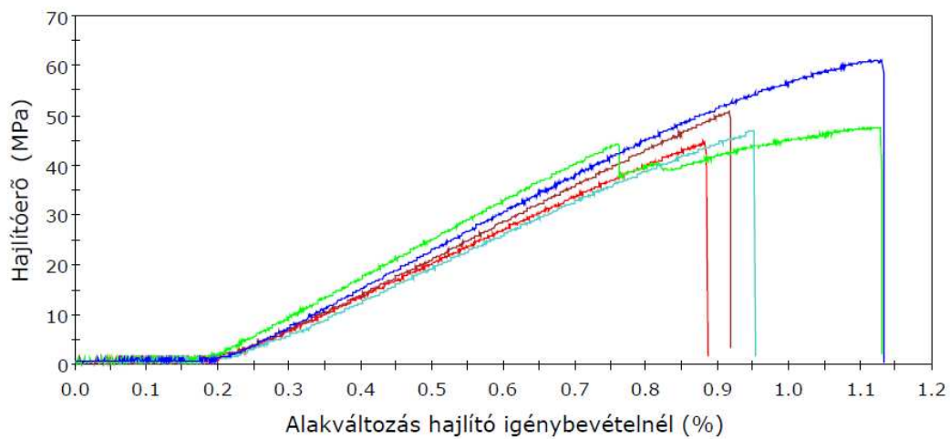
Flex Test
