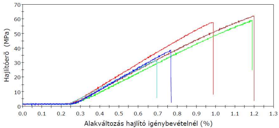
Flex Test
