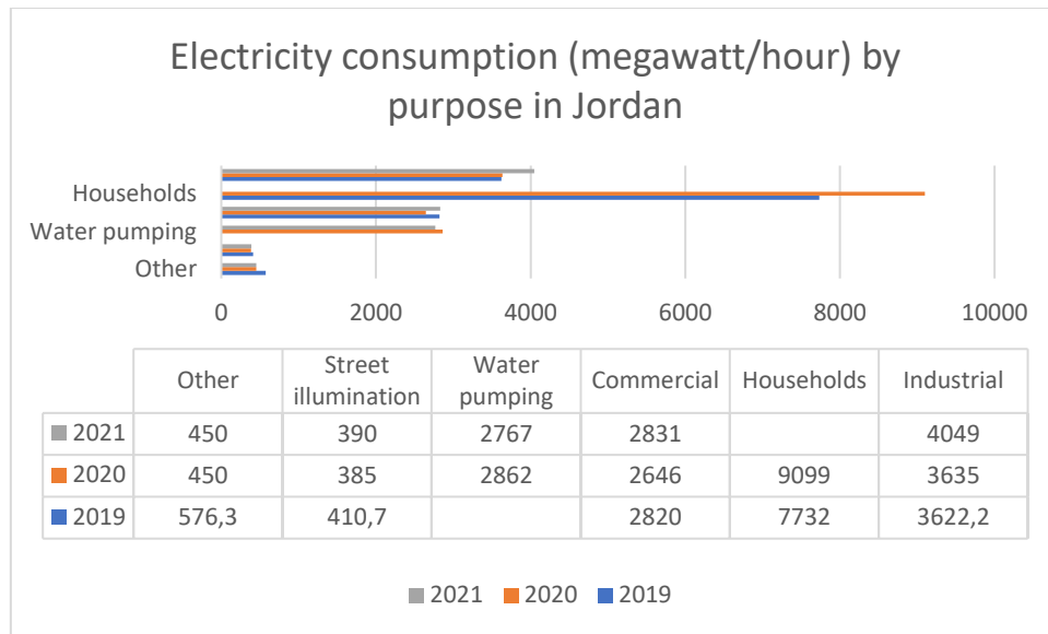
Figure 9 Electricity consumption (giga watt/hour) by purpose in Jordan source (statisces department of jordan reports 2019-2022)
