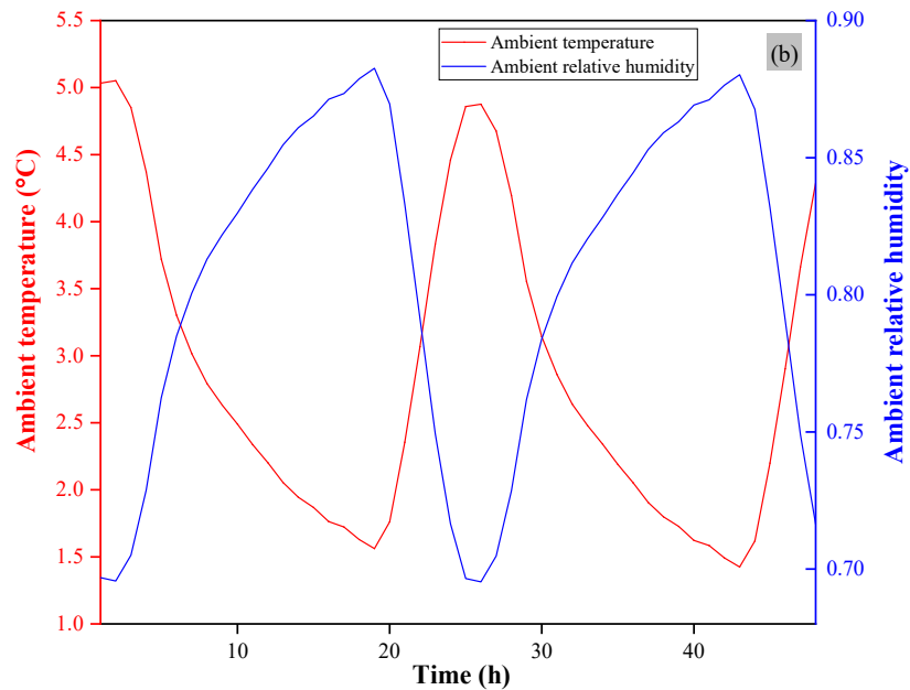
Figure 2.14 Ambient data for temperature and relative humidity used on the exterior side of the wall: (a) summertime; (b) wintertime.
