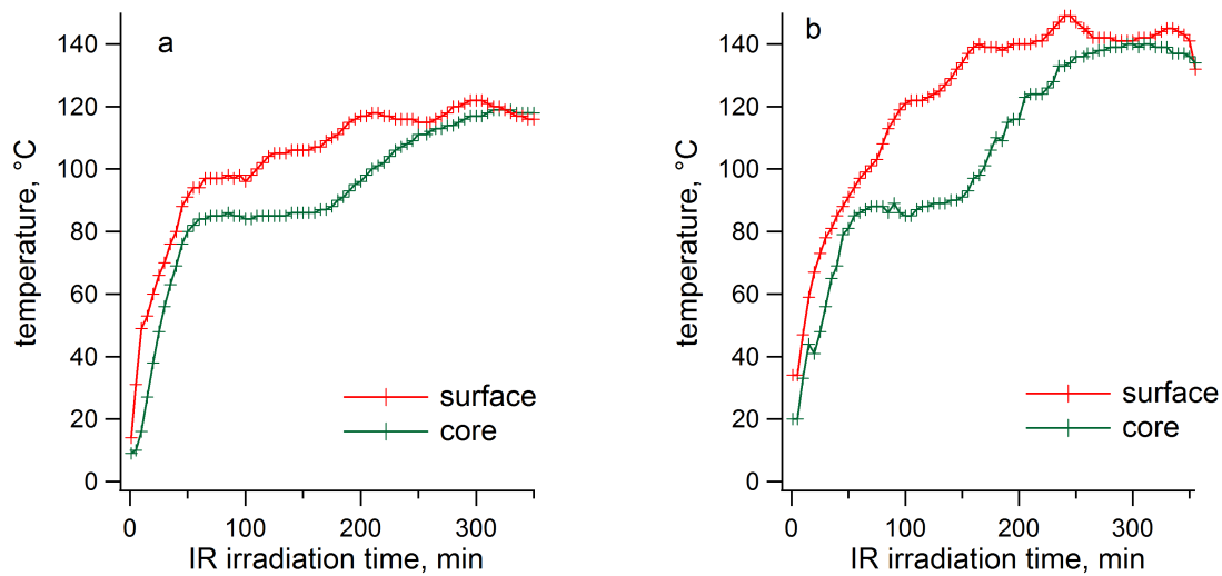
(a) Maximum temperature of the IR emitters were set to 140 °C (b) The temperature of the IR emitters was increased throughout the IR irradiation process to a maximal 170 °C
