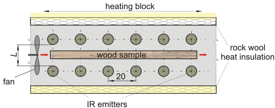
Figure 5.2. Horizontal cross-section of the IR furnace. The distance between the emitters is given in cm dimension
