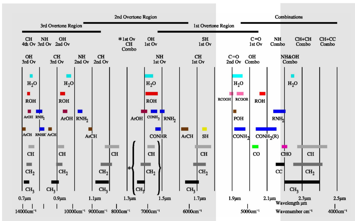
Figure 10.2. Major analytical bands and relative peak positions for prominent near-infrared absorptions.
