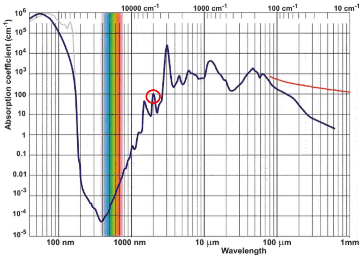
Figure 10.3. Absorption coefficients for water. The absorption spectrum of liquid water http://www.lsbu.ac.uk/water/vibrat.html
