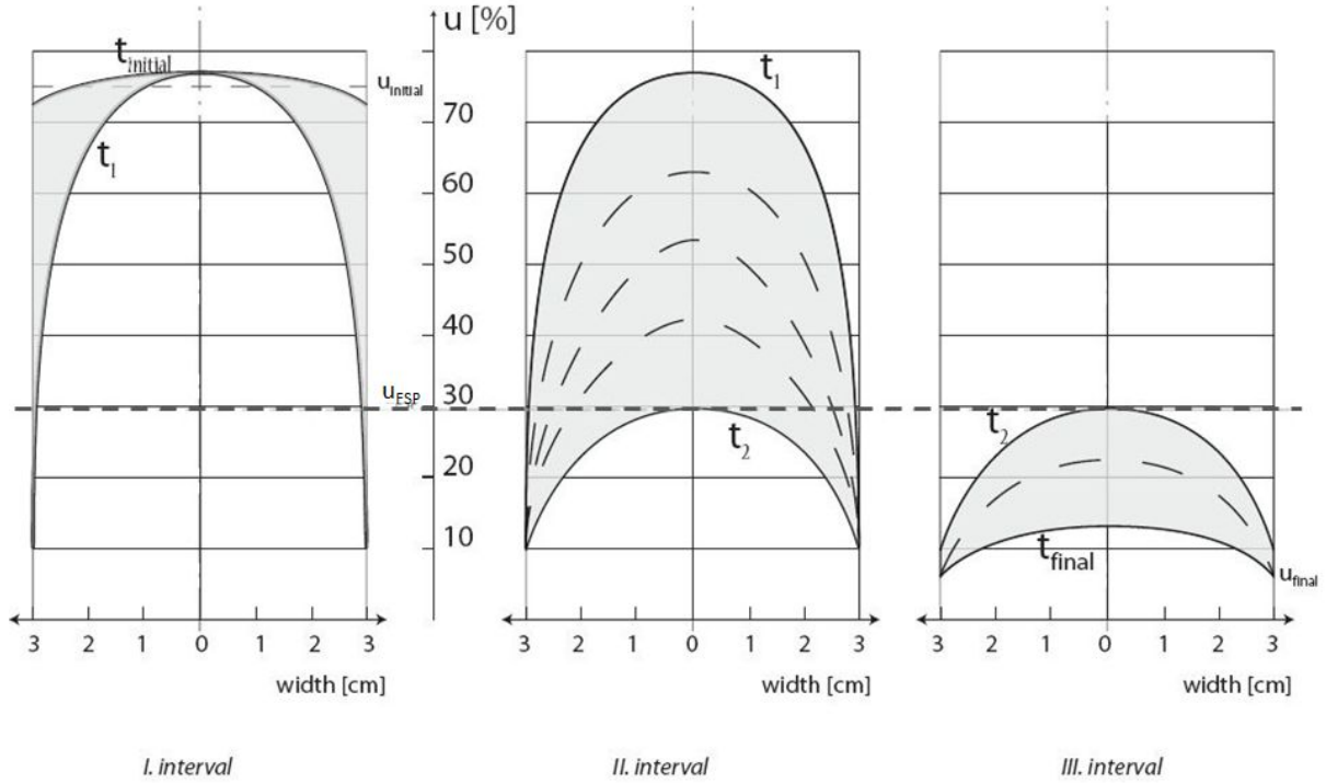
Figure 3.7. The change of MC perpendicular to the surface of a wood sample during the drying intervals according to Imre 1974. The notation u_{initial} is the initial MC, u_{final} is the final MC, while t , with different subscripts, refers to the drying time intervals. The dashed line around 30% of MC refers to the u_{FSP} , which is the MC at the fiber saturation point (FSP)
