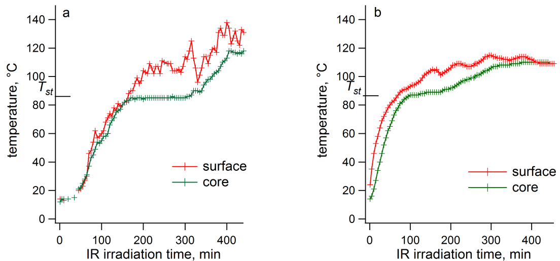
(a) Maximum emitter temperature was set to 165°C
