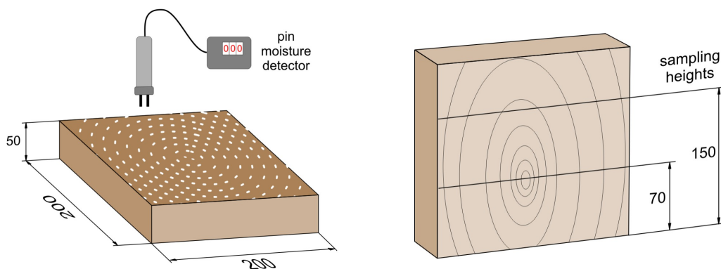
(a) A set of concentric circles centered around the pith with 10 mm radius difference defined for measuring moisture distribution (b) The two heights of sampling along the cross-line at 70 mm above the bottom (at pith height) and at 150 mm above the bottom
